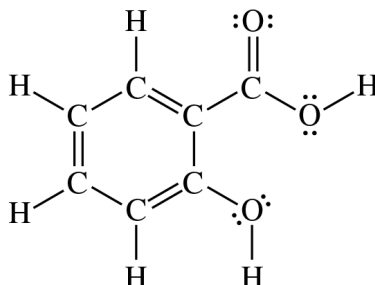
Salicylic Acid Melting Point: 159°C
