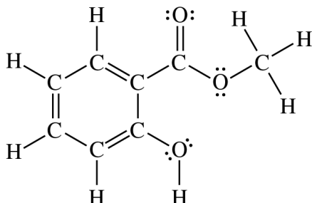
Methyl Salicylate Melting Point: -9°C
